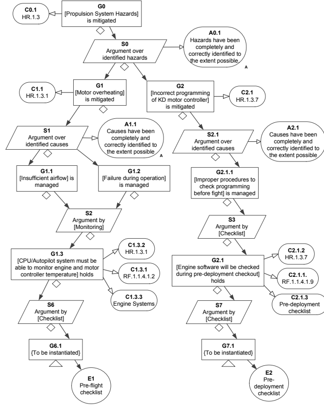
Fig. 3. Fragment of the Swift UAS safety case (in GSN) obtained by transformation of the hazards table and the functional requirements table
