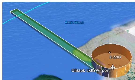
(b) 3-D visualization of the transit corridor overlapping the restricted airspace R-2204 at the southern end, and extending beyond U.S. airspace in the northern end
