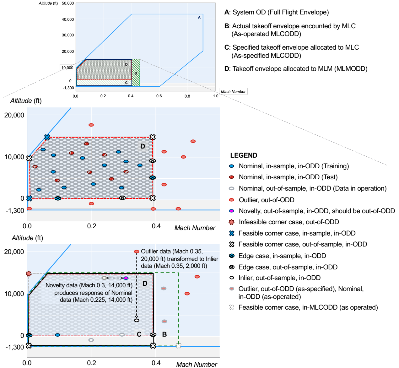
Figure 1: An example flight envelope (region A) representing an aircraft system OD, whose refinement and allocation to an MLC and MLM give, respectively, an As-operated MLCODD (region B), containing an As-specified MLCODD (region C), itself containing the MLMODD (region D), for the takeoff regime. The shapes representing the different ODDs are practically congruent, but have been shown slightly offset here to differentiate each from the other. Zoomed-in views of the respective ODDs highlight the different categories and kinds of data used to characterize them.
